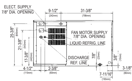
REMOTE AIR-COOLED UNIT
